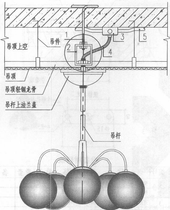
杆式吊灯在吊顶下安装
