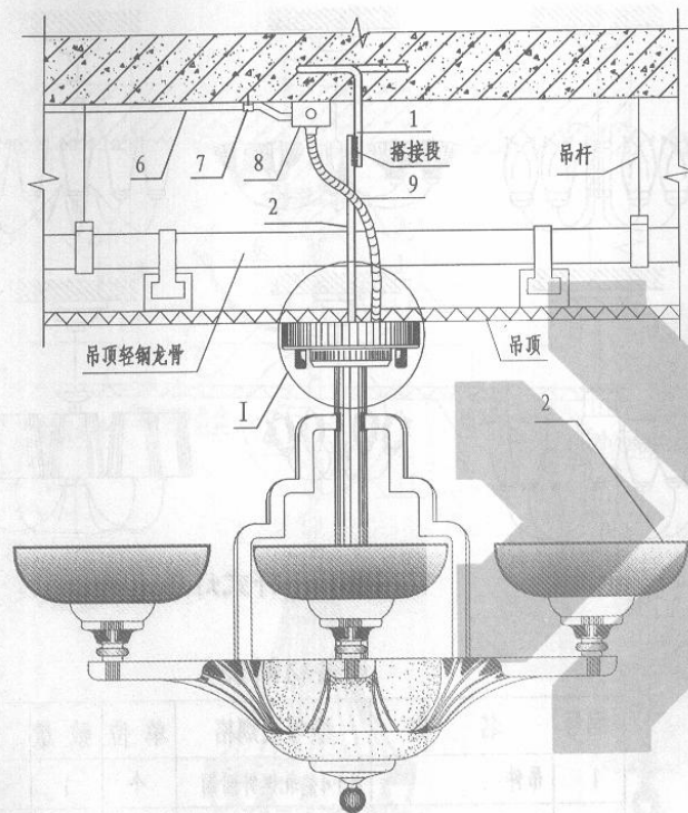
杆式吊灯在吊顶下安装
