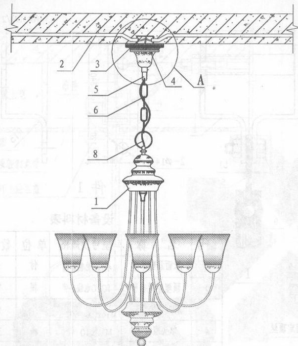
链式吊灯在顶板下安装
